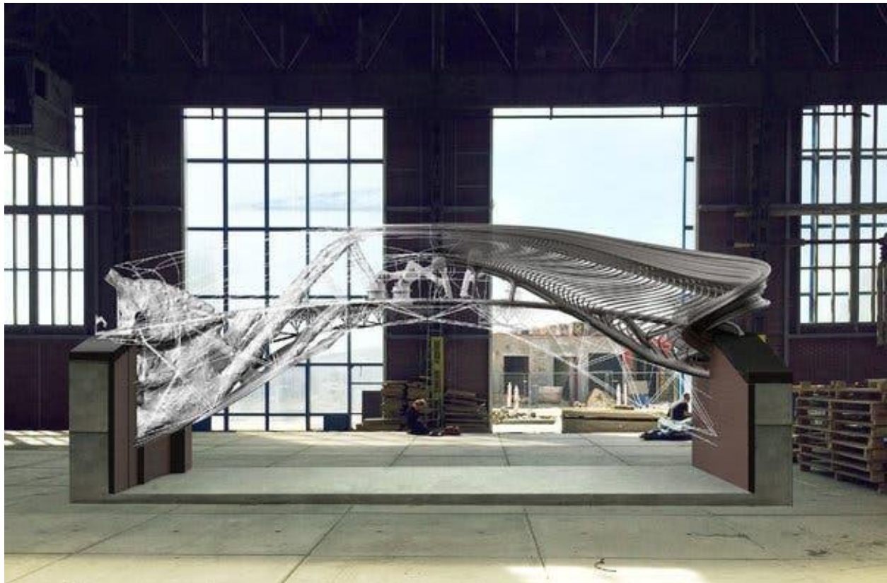
A rendering of the MX3D Bridge in the workshop. The bridge is being executed by robotic 3-D printers and will be completed in 2018. It will span an old canal in Amsterdam, connecting the technology of the future with the city's past. Credit...Joris Laarman Lab
